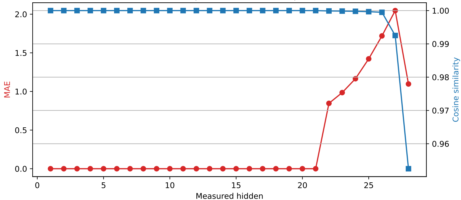
Qwen2.5-7B-Instruct | Quantized layer 21 | float64 \rightarrow int2
