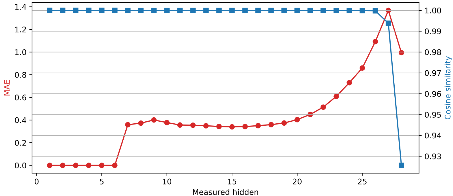
Qwen2.5-7B-Instruct | Quantized layer 6 | float64 → int2
