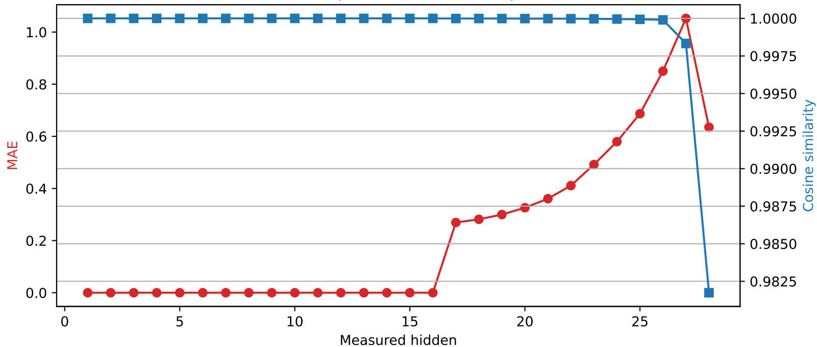
Qwen2.5-7B-Instruct | Quantized layer 16 | float64 → int2
