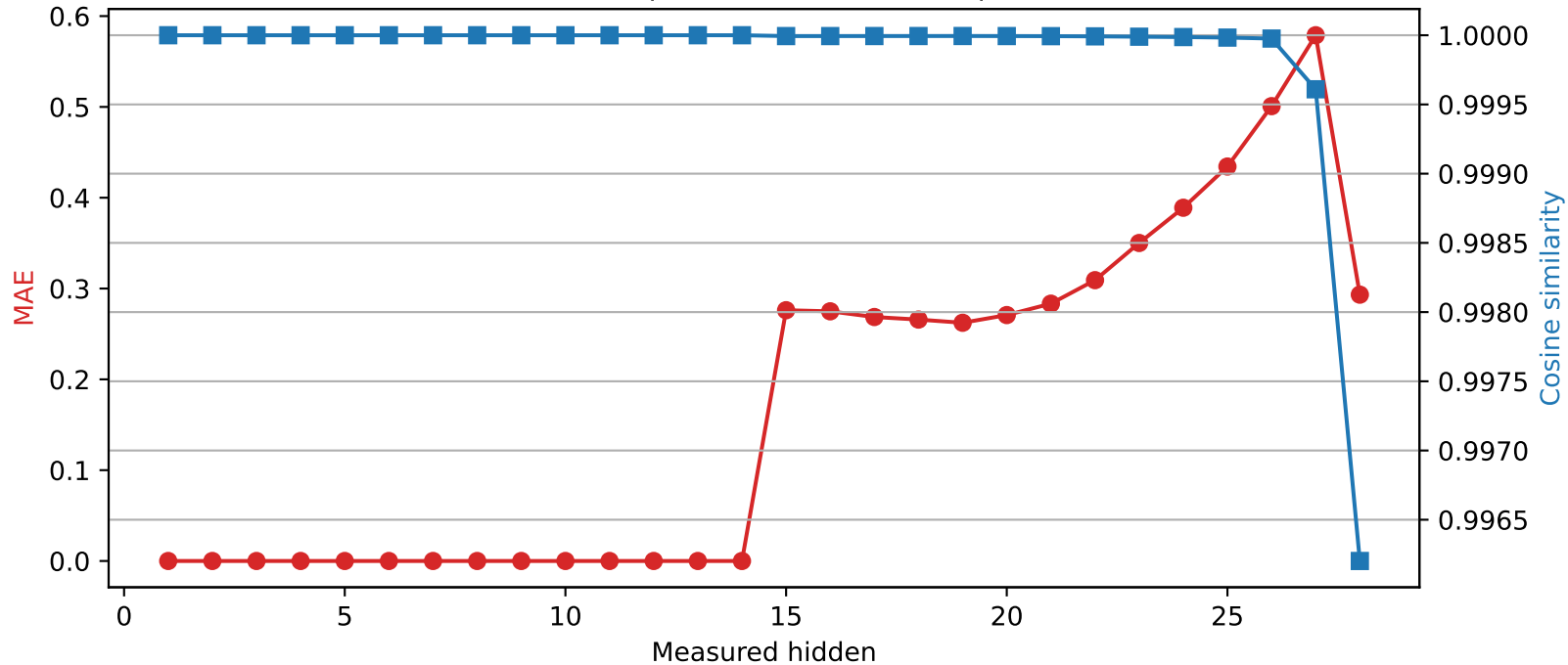
Qwen2.5-7B-Instruct | Quantized layer 14 | float64 → int2
