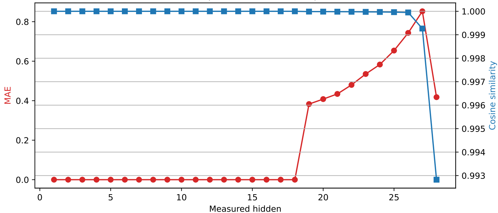
Qwen2.5-7B-Instruct | Quantized layer 18 | float64 → int2
