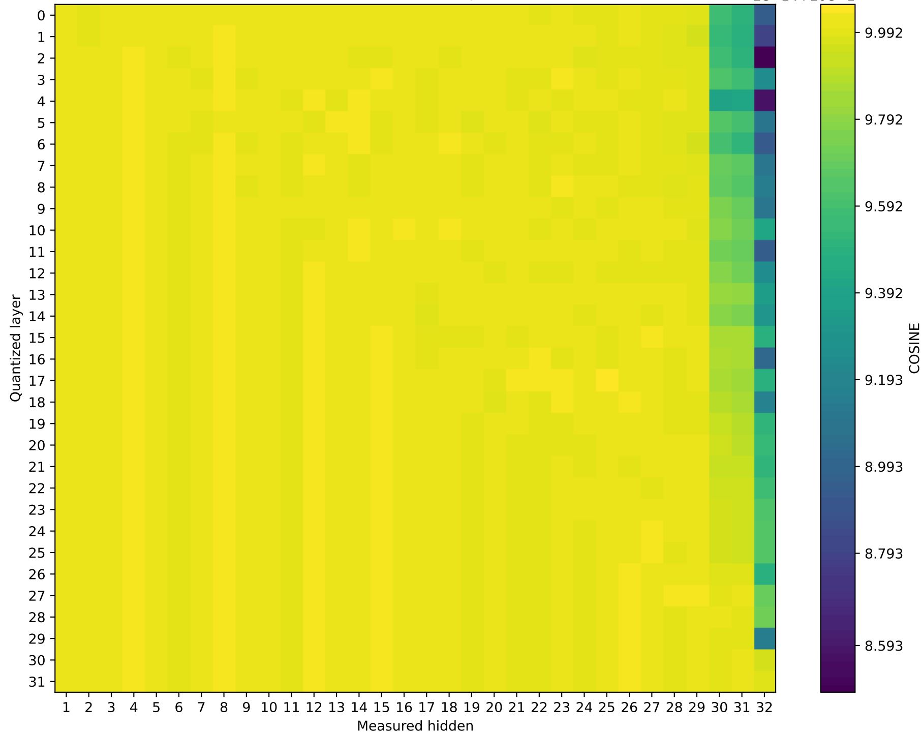
Model: Phi-3-mini-4k-instruct | float64 → int32
