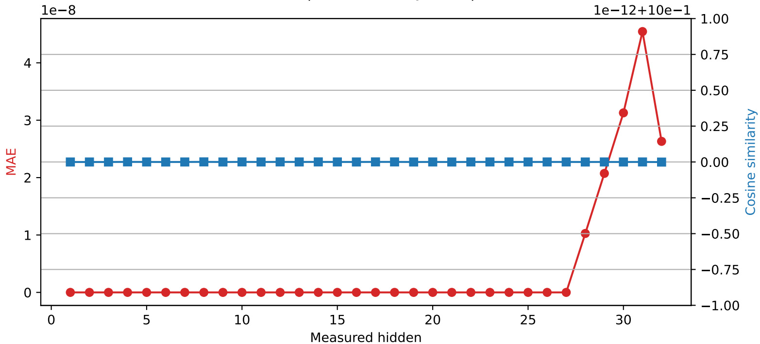
Phi-3-mini-4k-instruct | Quantized layer 27 | float64 → int32
