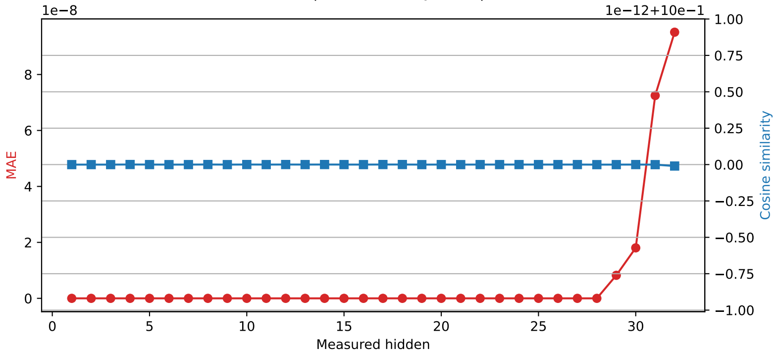
Phi-3-mini-4k-instruct | Quantized layer 28 | float64 → int32
