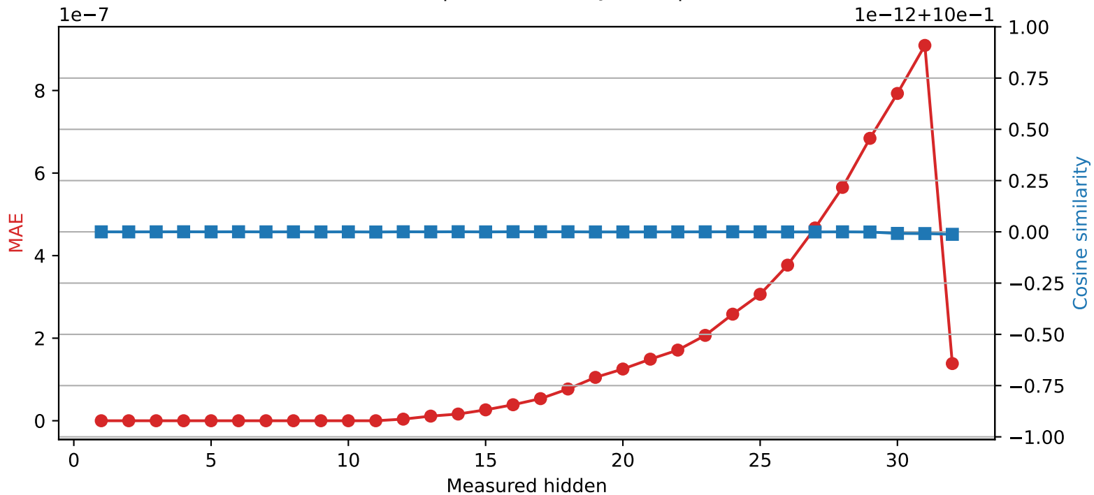
Phi-3-mini-4k-instruct | Quantized layer 11 | float64 → int32
