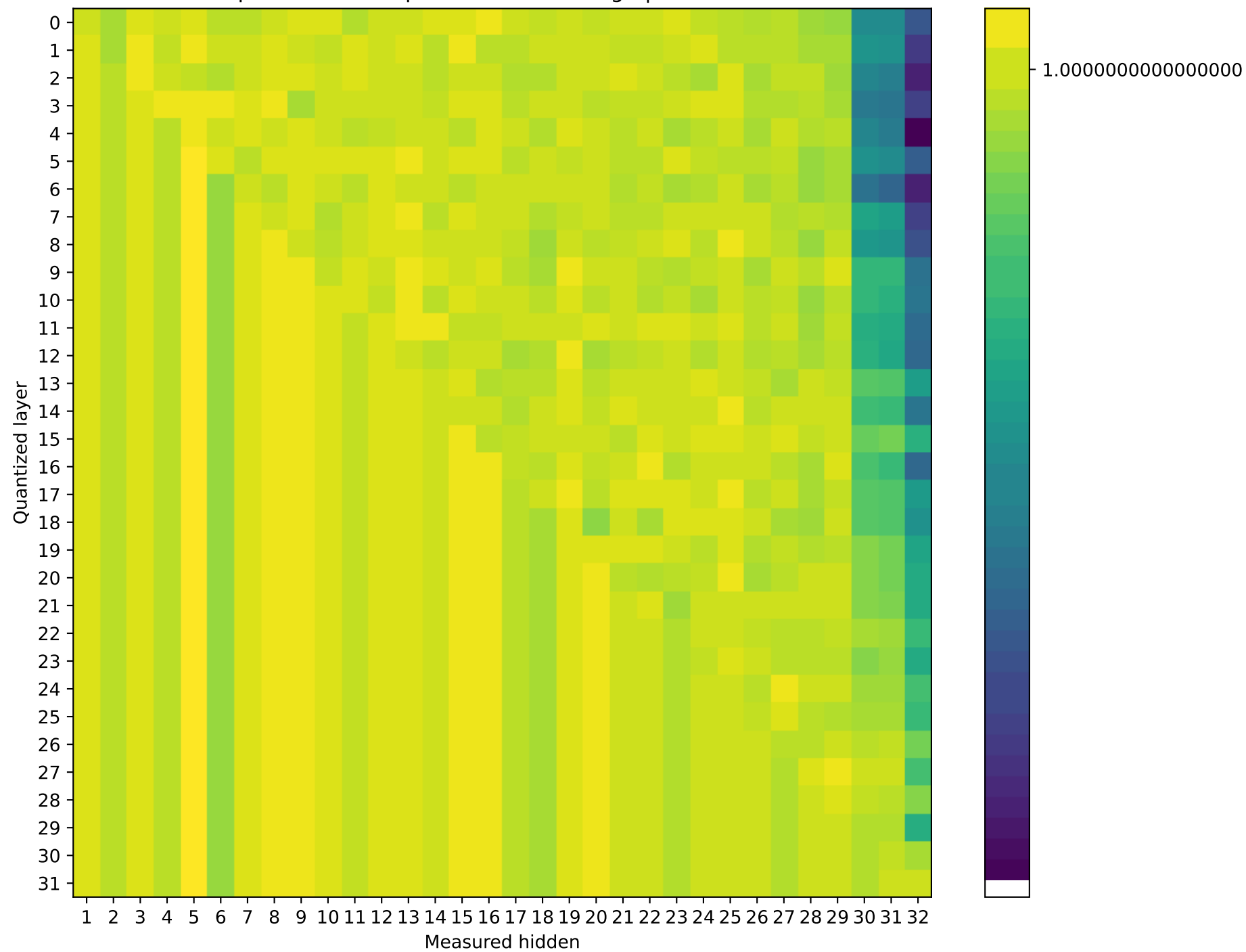
Phi-3-mini-4k-instruct Prompt 2: cos sim representation damage | float64 → int32
