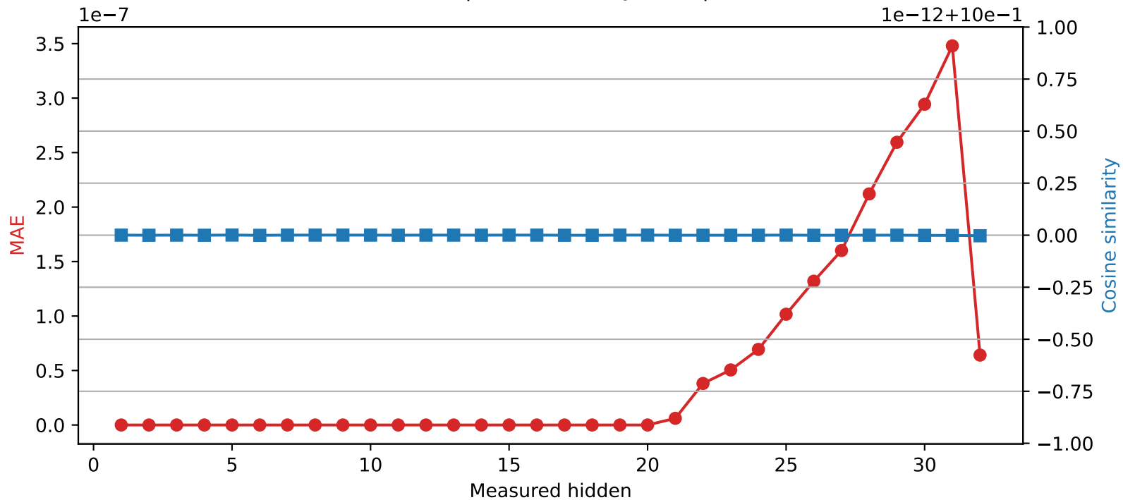
Phi-3-mini-4k-instruct | Quantized layer 20 | float64 → int32
