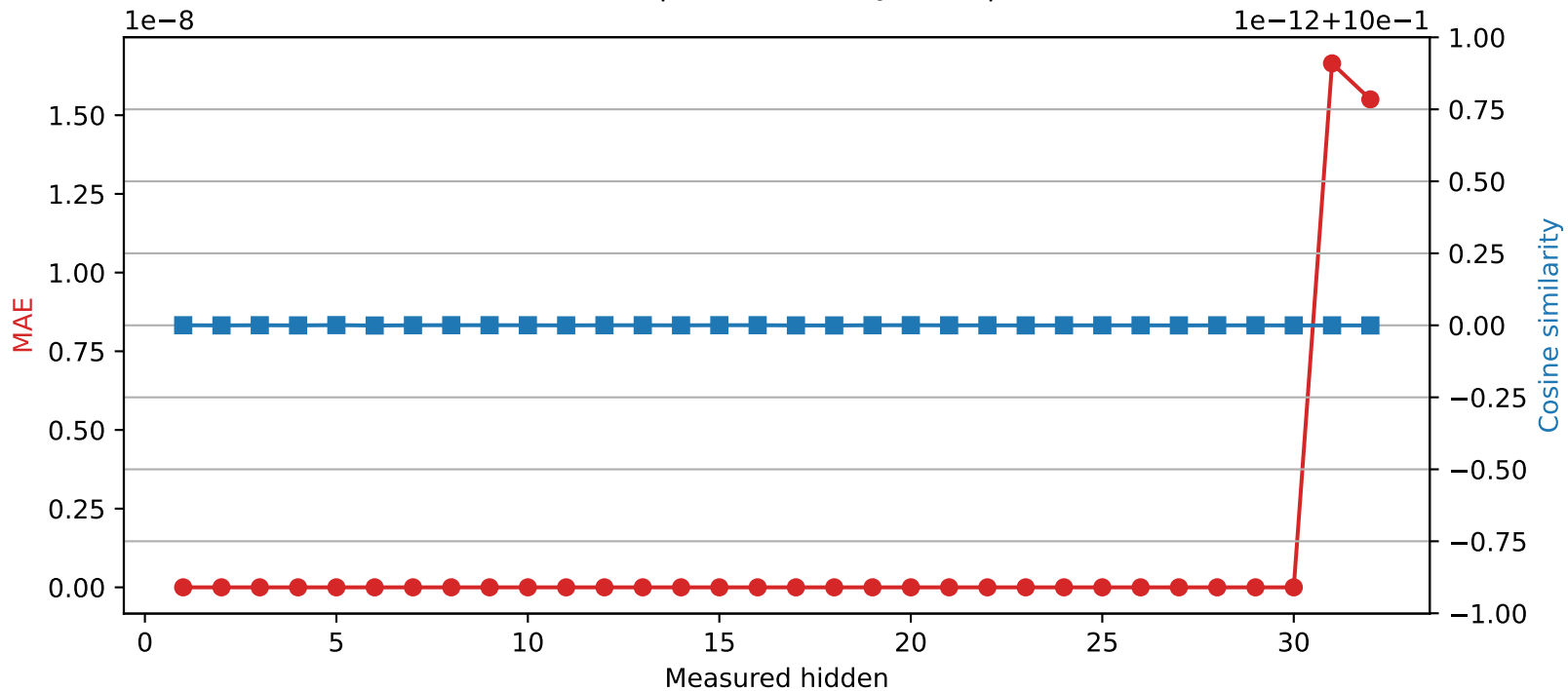
Phi-3-mini-4k-instruct | Quantized layer 30 | float64 → int32
