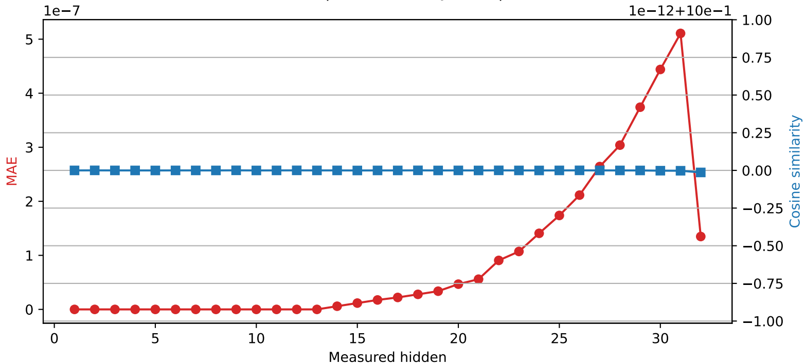
Phi-3-mini-4k-instruct | Quantized layer 13 | float64 → int32
