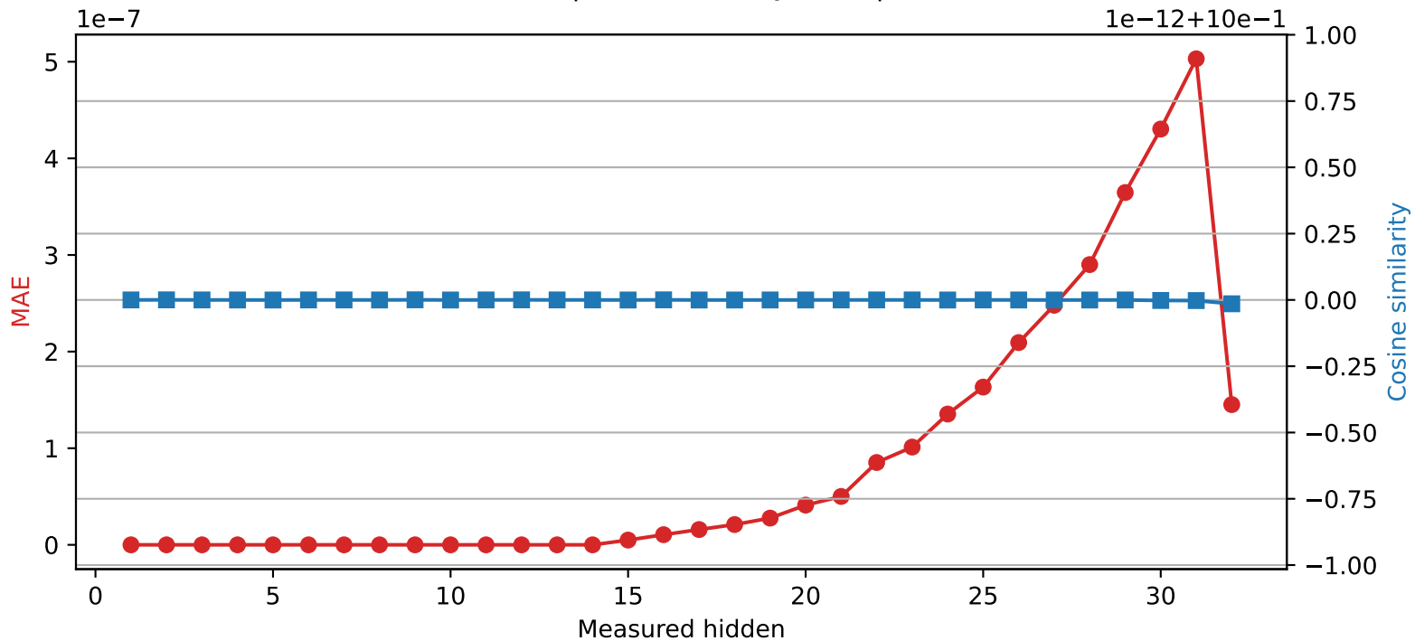
Phi-3-mini-4k-instruct | Quantized layer 14 | float64 → int32
