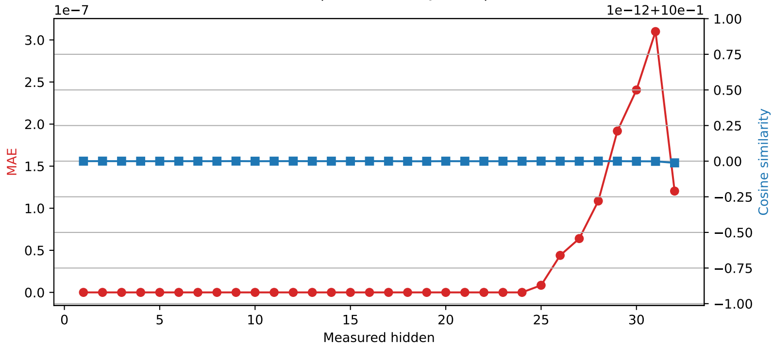
Phi-3-mini-4k-instruct | Quantized layer 24 | float64 → int32
