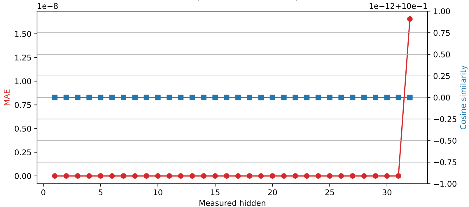
Phi-3-mini-4k-instruct | Quantized layer 31 | float64 → int32
