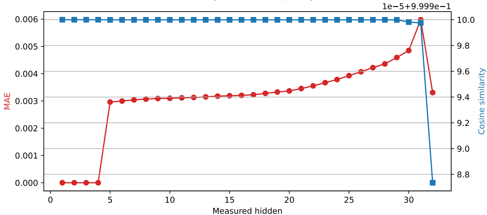
Phi-3-mini-4k-instruct | Quantized layer 4 | float32 → int16
