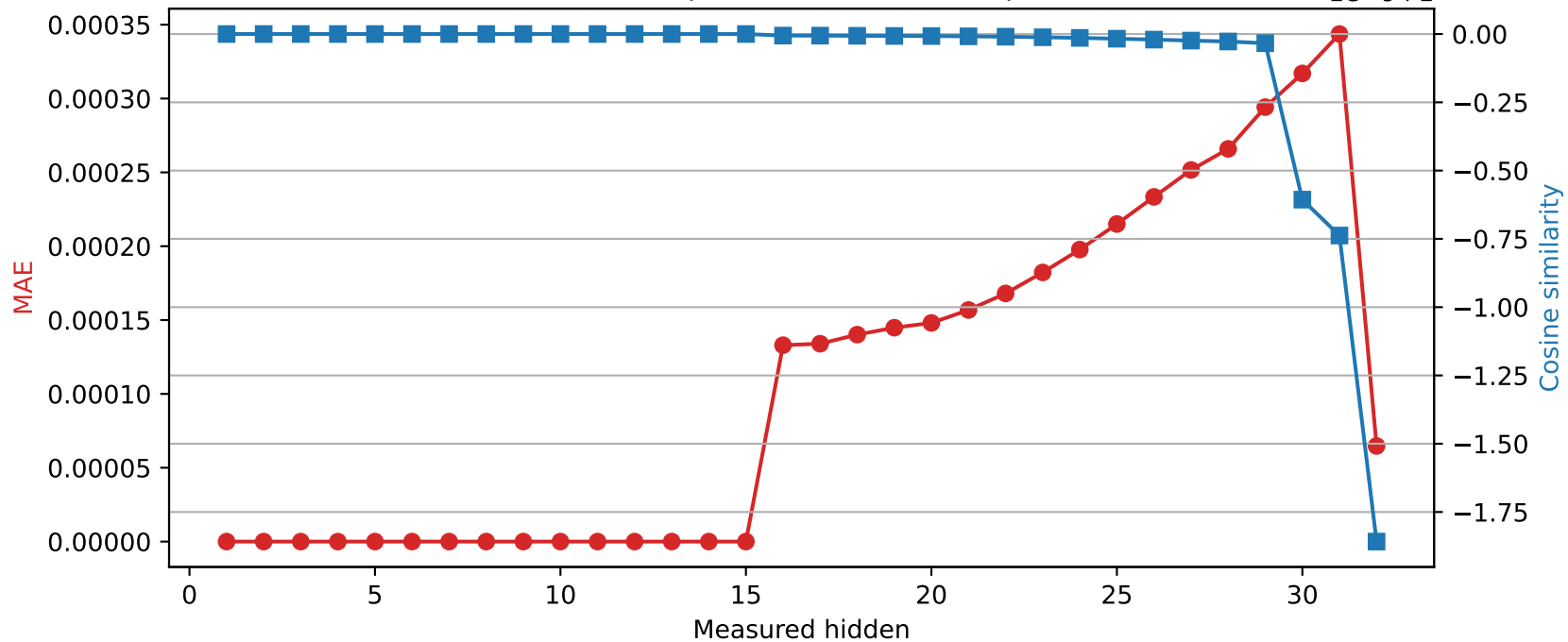
Phi-3-mini-4k-instruct | Quantized layer 15 | float32 → int16
