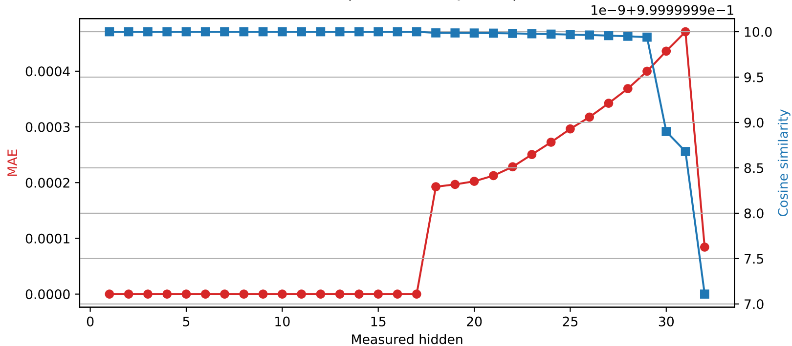
Phi-3-mini-4k-instruct | Quantized layer 17 | float32 → int16
