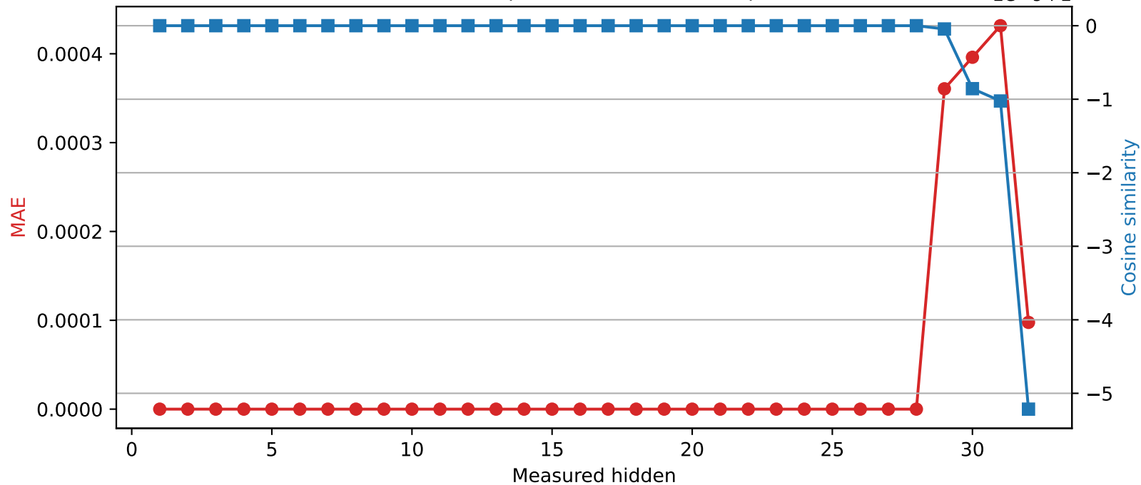
Phi-3-mini-4k-instruct | Quantized layer 28 | float32 \rightarrow int16
