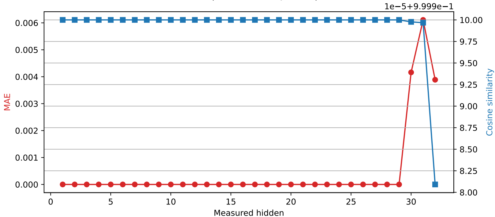
Phi-3-mini-4k-instruct | Quantized layer 29 | float32 → int16
