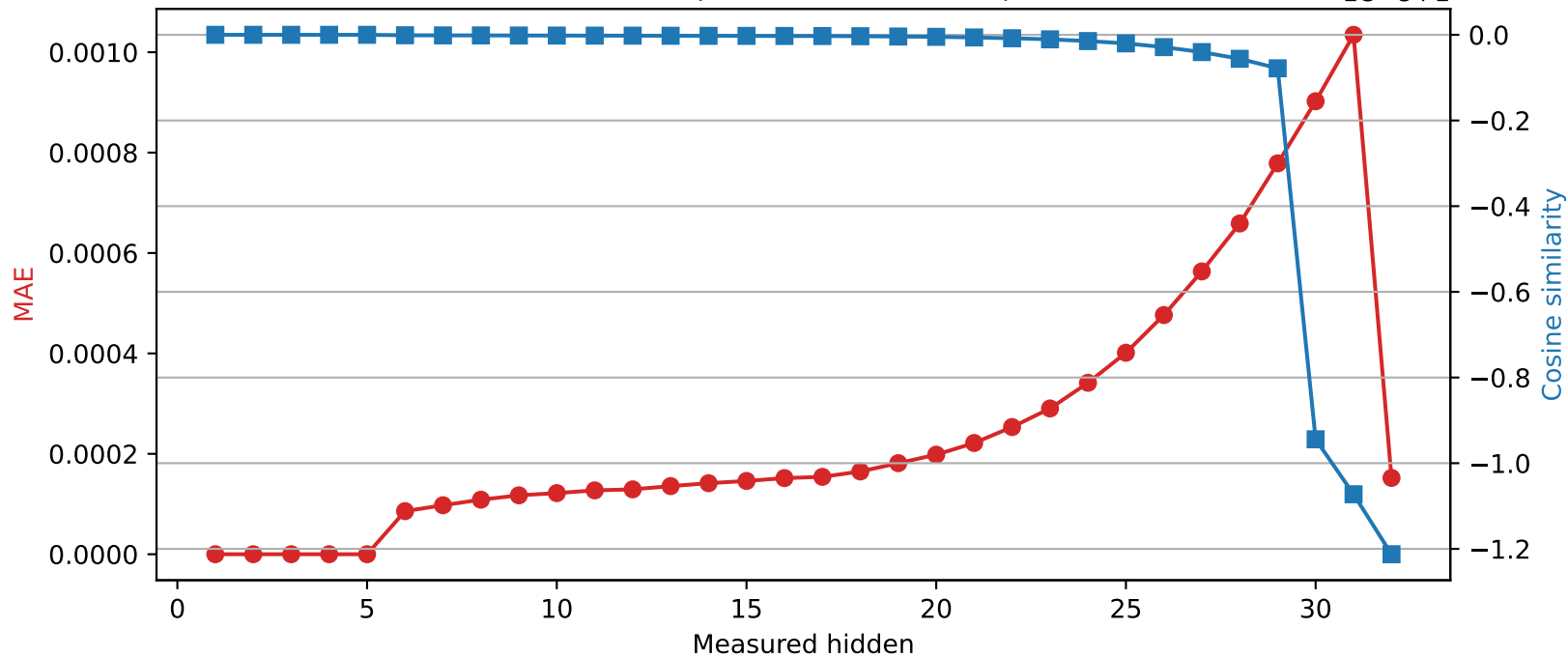
Phi-3-mini-4k-instruct | Quantized layer 5 | float32 \rightarrow int16
