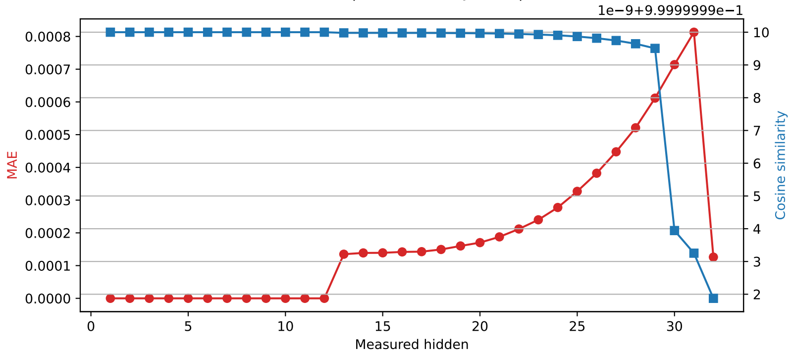
Phi-3-mini-4k-instruct | Quantized layer 12 | float32 \rightarrow int16
