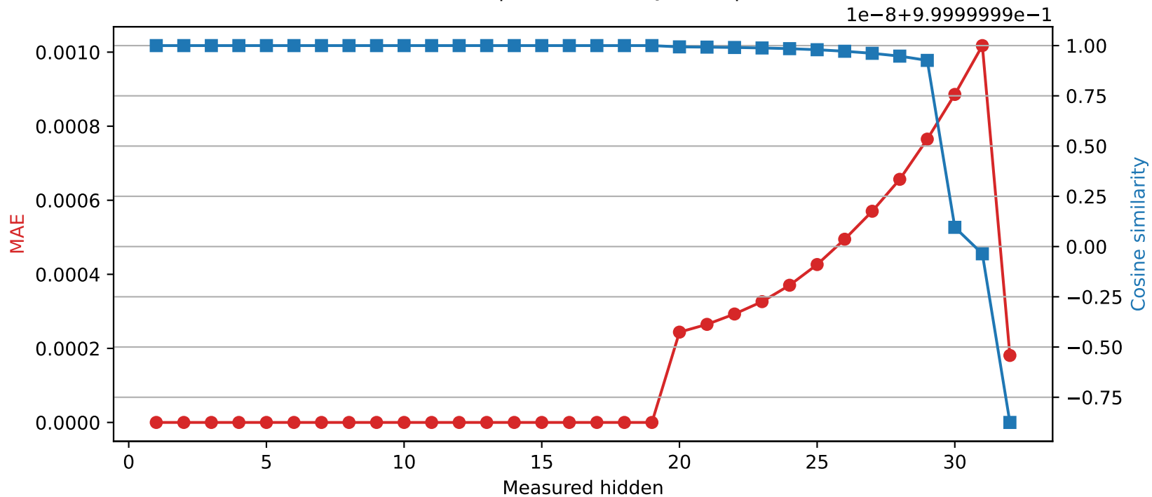
Phi-3-mini-4k-instruct | Quantized layer 19 | float32 → int16
