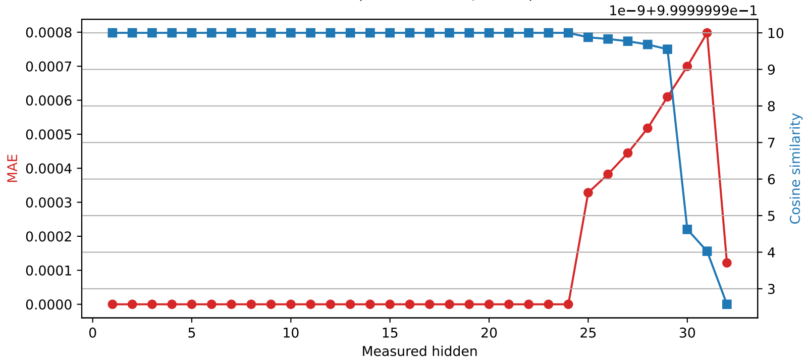
Phi-3-mini-4k-instruct | Quantized layer 24 | float32 → int16
