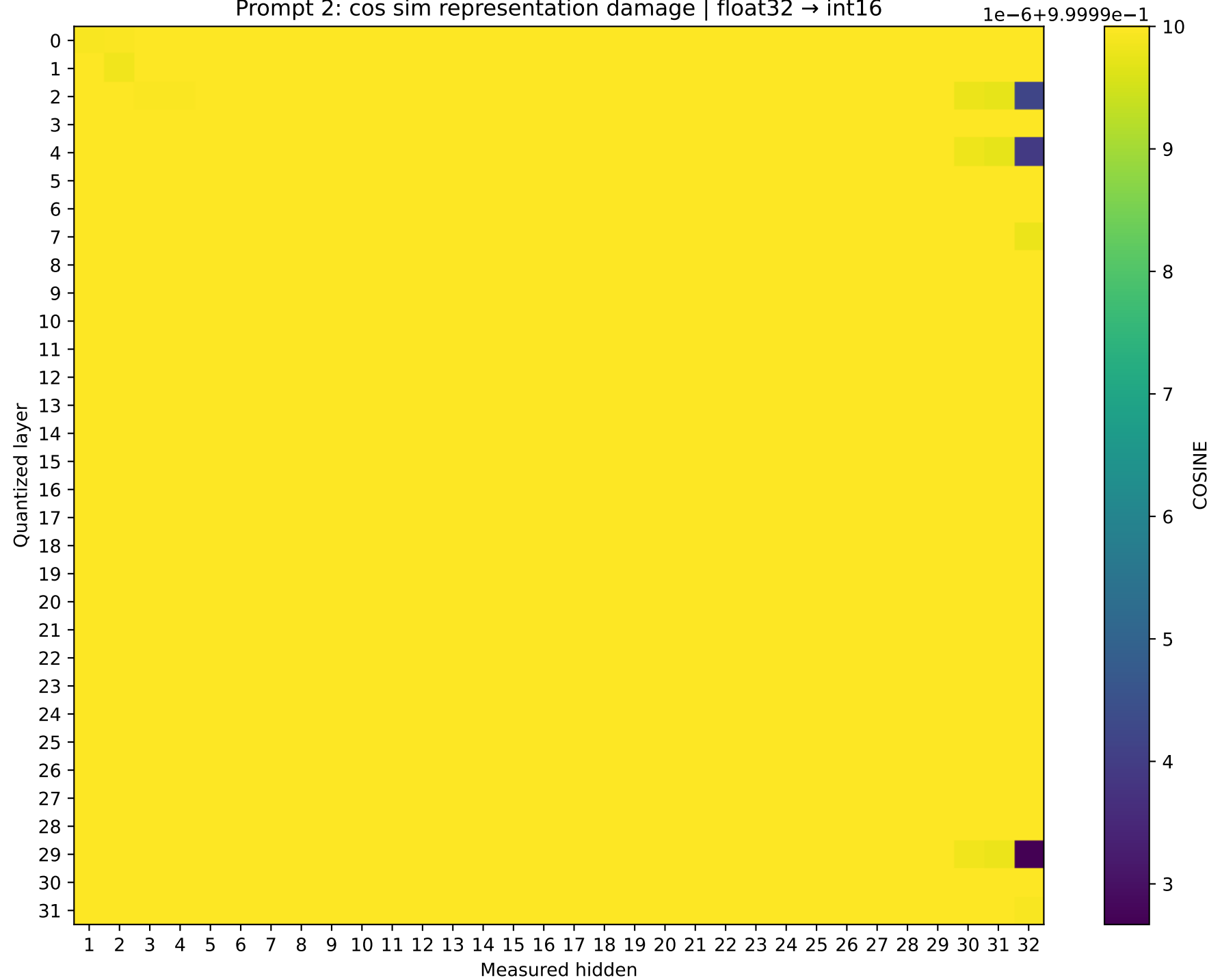
Phi-3-mini-4k-instruct Prompt 2: cos sim representation damage | float32 → int16
