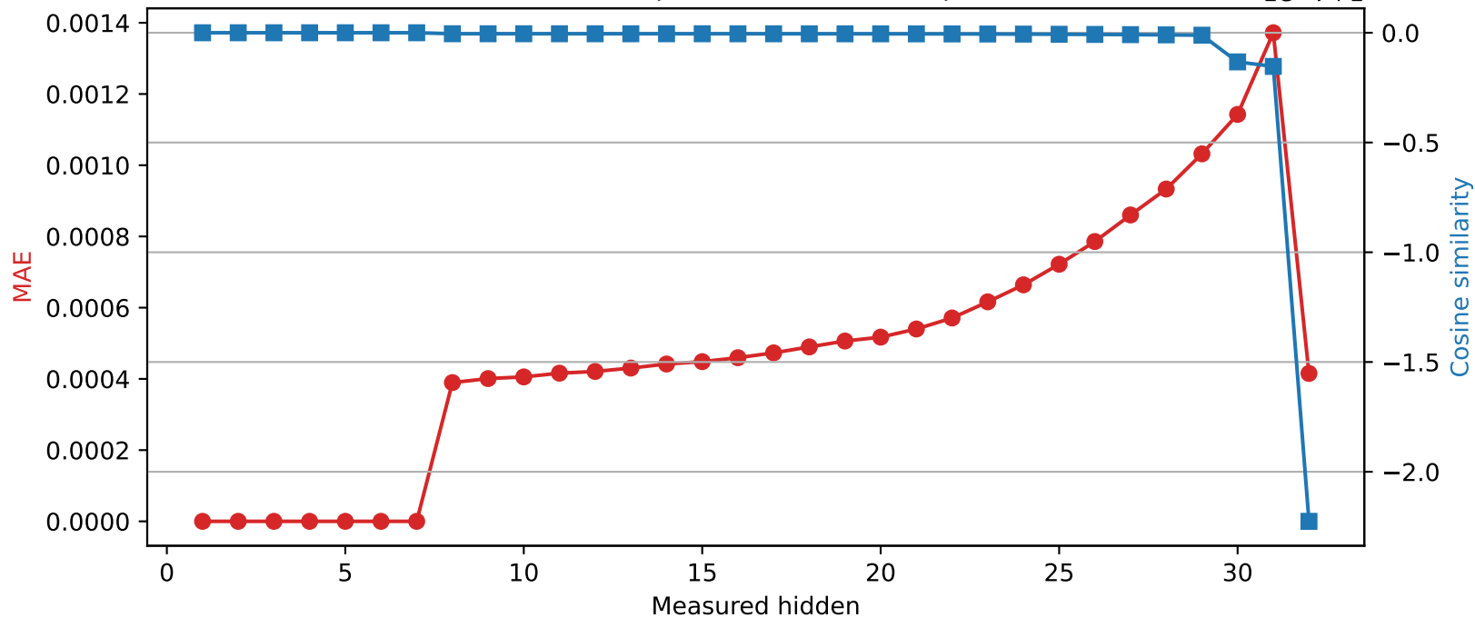
Phi-3-mini-4k-instruct | Quantized layer 7 | float32 \rightarrow int16
