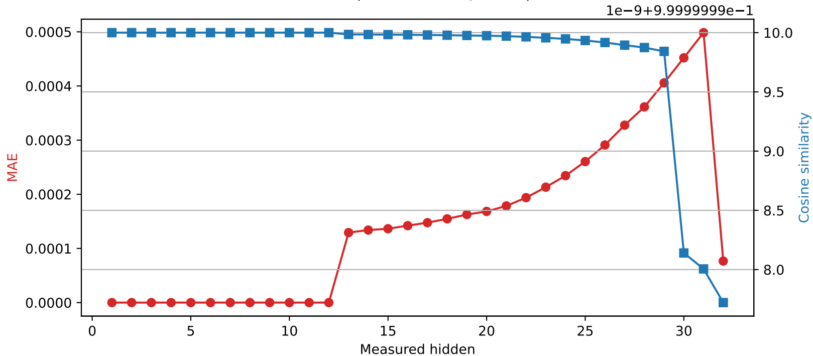
Phi-3-mini-4k-instruct | Quantized layer 12 | float32 \rightarrow int16
