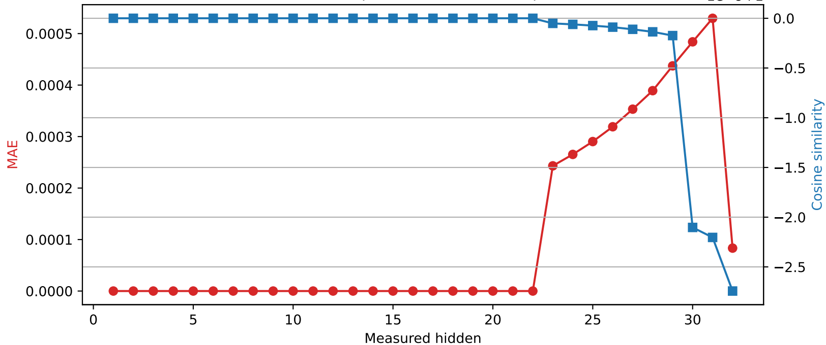
Phi-3-mini-4k-instruct | Quantized layer 22 | float32 \rightarrow int16
