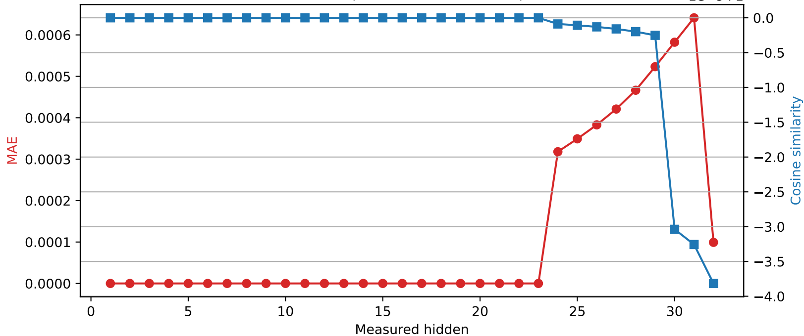
Phi-3-mini-4k-instruct | Quantized layer 23 | float32 → int16
