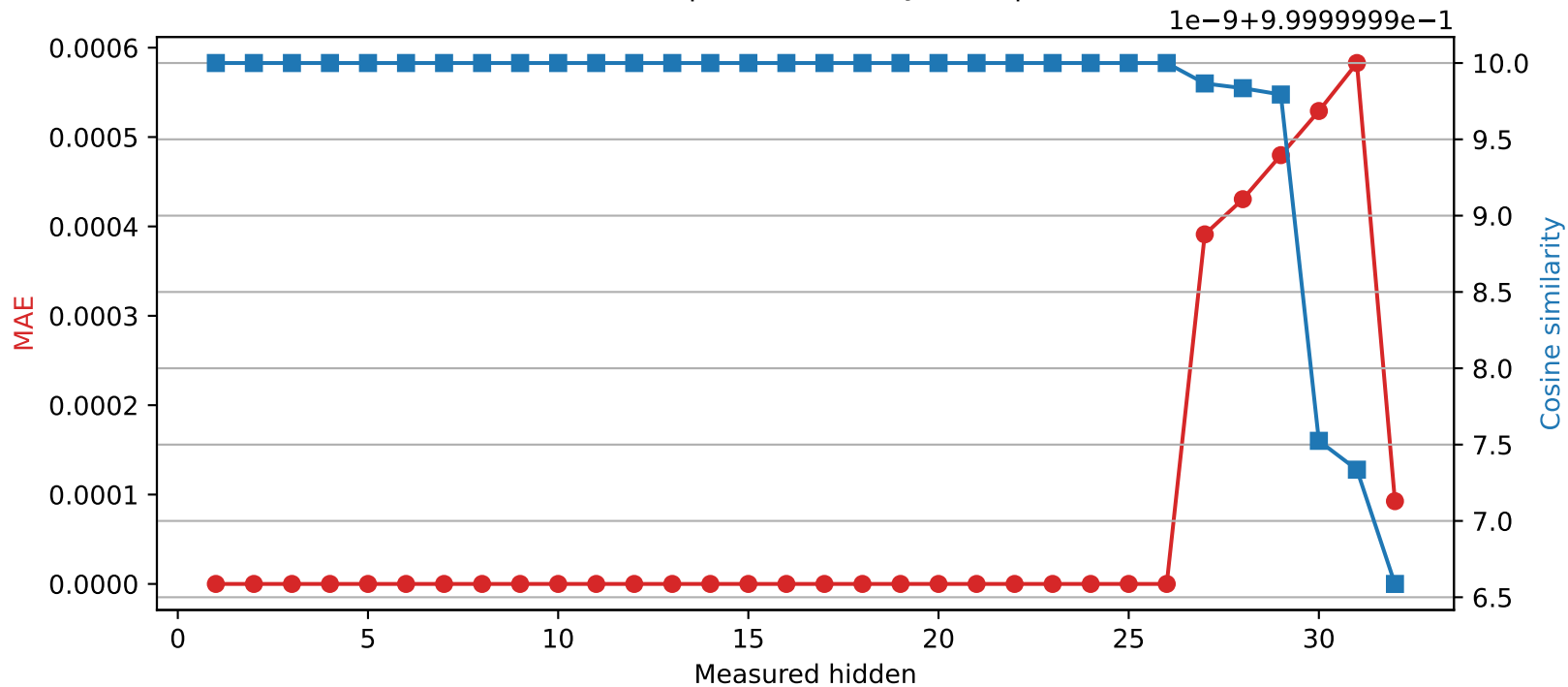
Phi-3-mini-4k-instruct | Quantized layer 26 | float32 → int16
