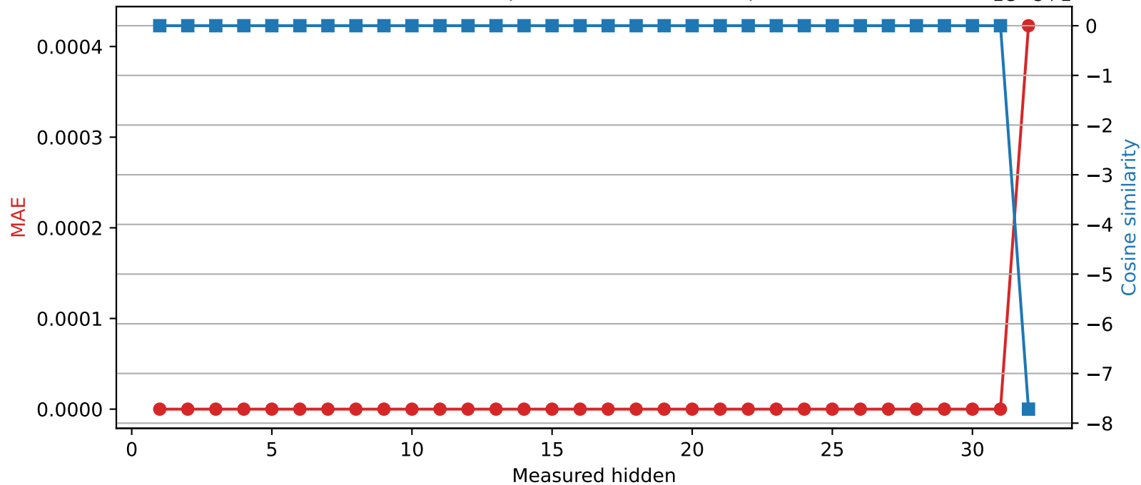
Phi-3-mini-4k-instruct | Quantized layer 31 | float32 \rightarrow int16
