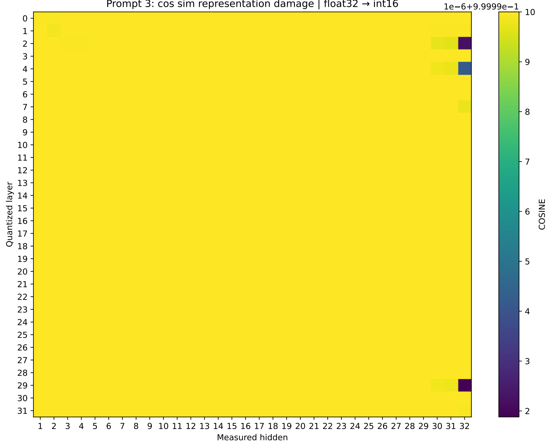
Phi-3-mini-4k-instruct Prompt 3: cos sim representation damage | float32 → int16
