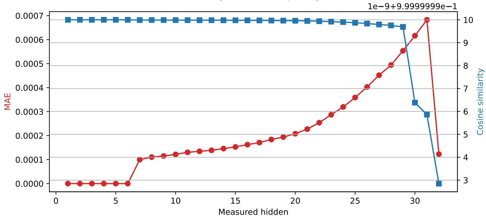
Phi-3-mini-4k-instruct | Quantized layer 6 | float32 → int16
