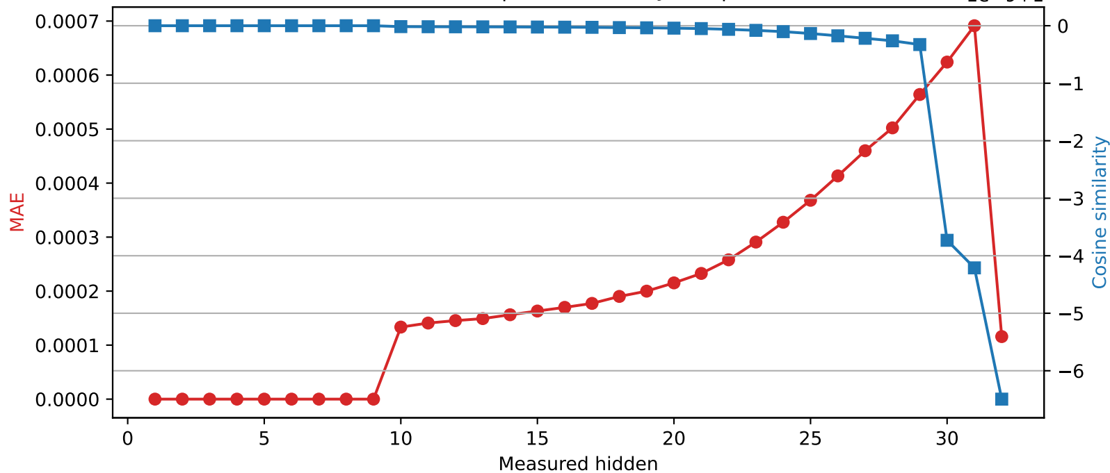
Phi-3-mini-4k-instruct | Quantized layer 9 | float32 → int16
