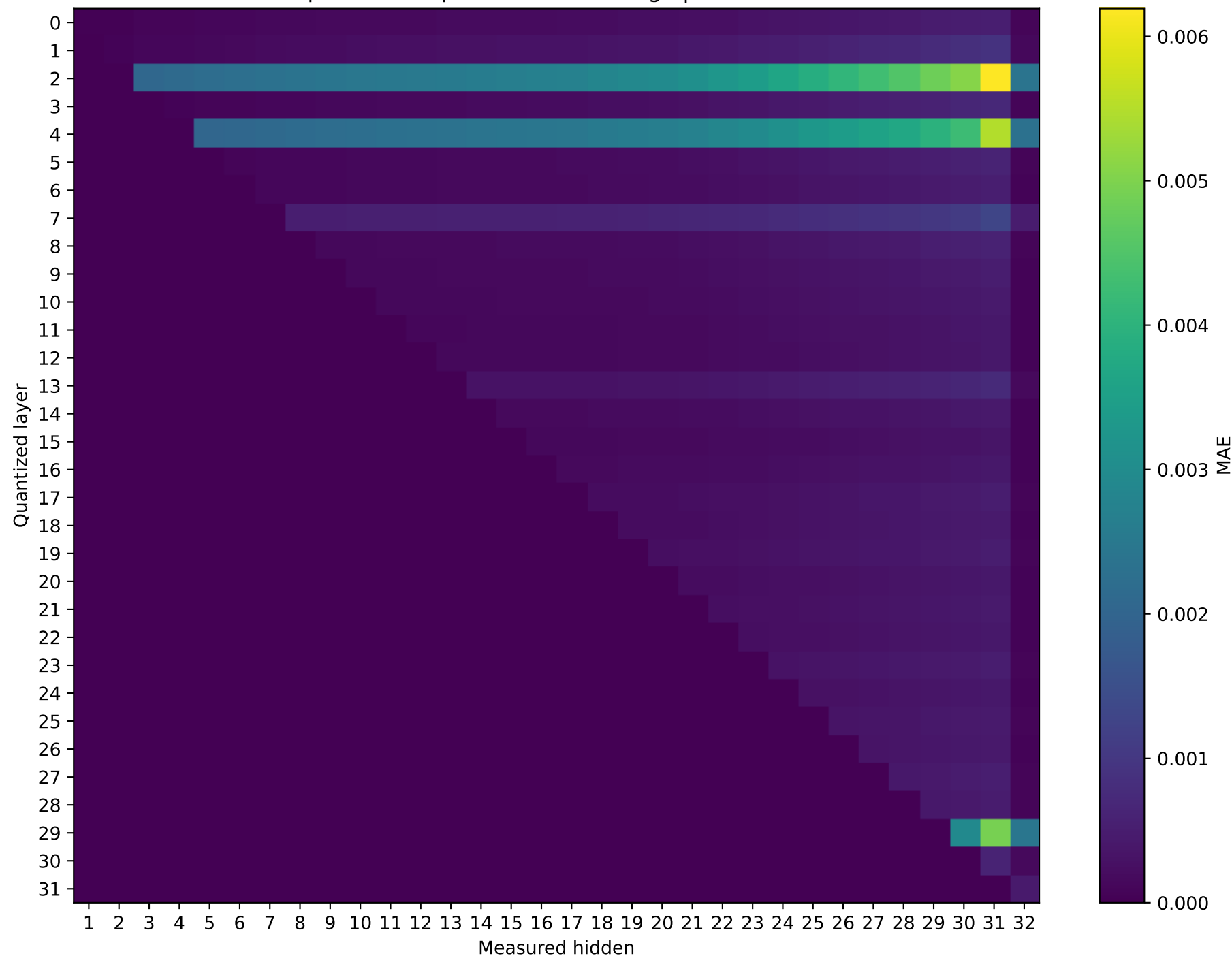
Phi-3-mini-4k-instruct Prompt 4: MAE representation damage | float32 \rightarrow int16
