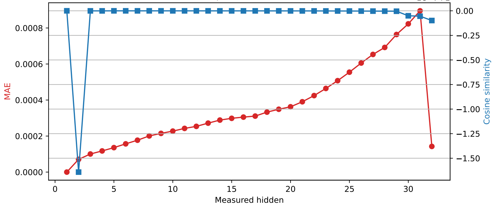
Phi-3-mini-4k-instruct | Quantized layer 1 | float32 \rightarrow int16
