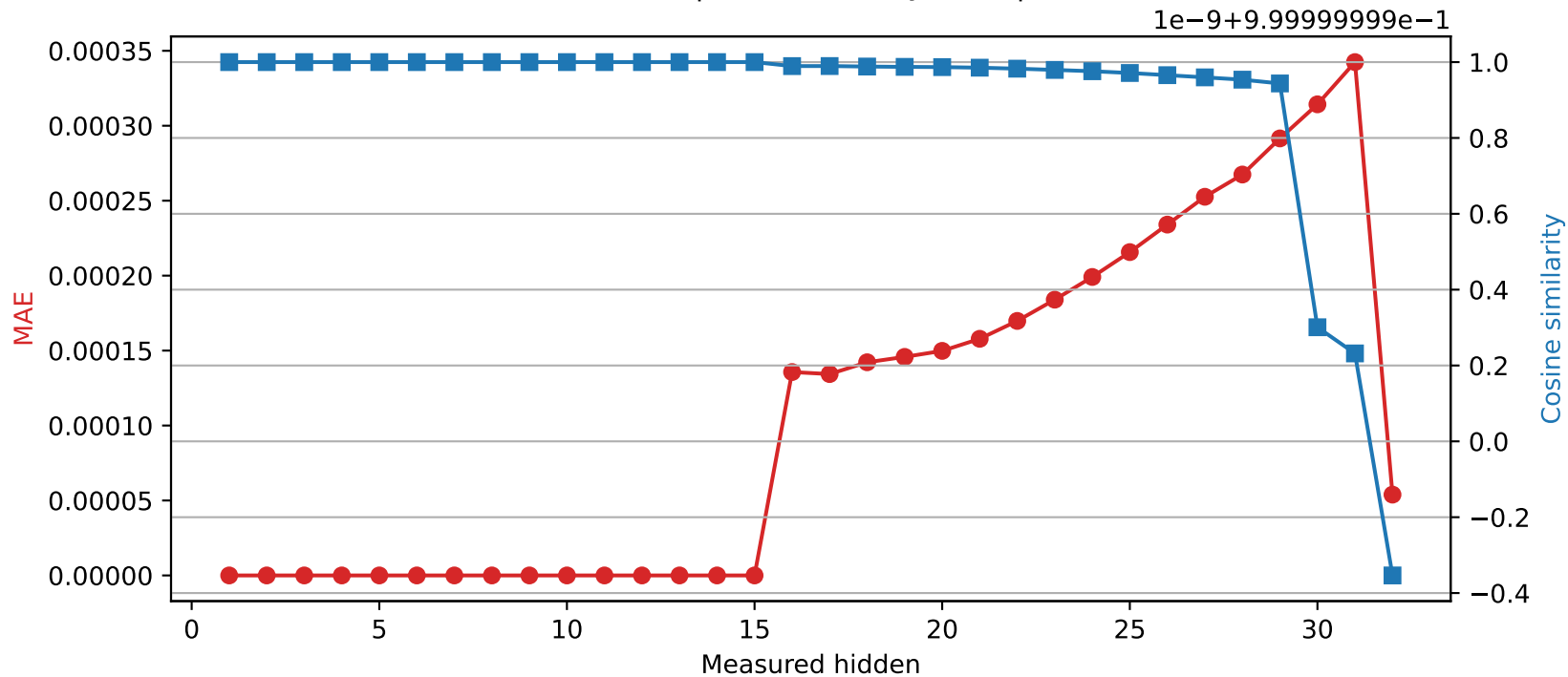
Phi-3-mini-4k-instruct | Quantized layer 15 | float32 \rightarrow int16
