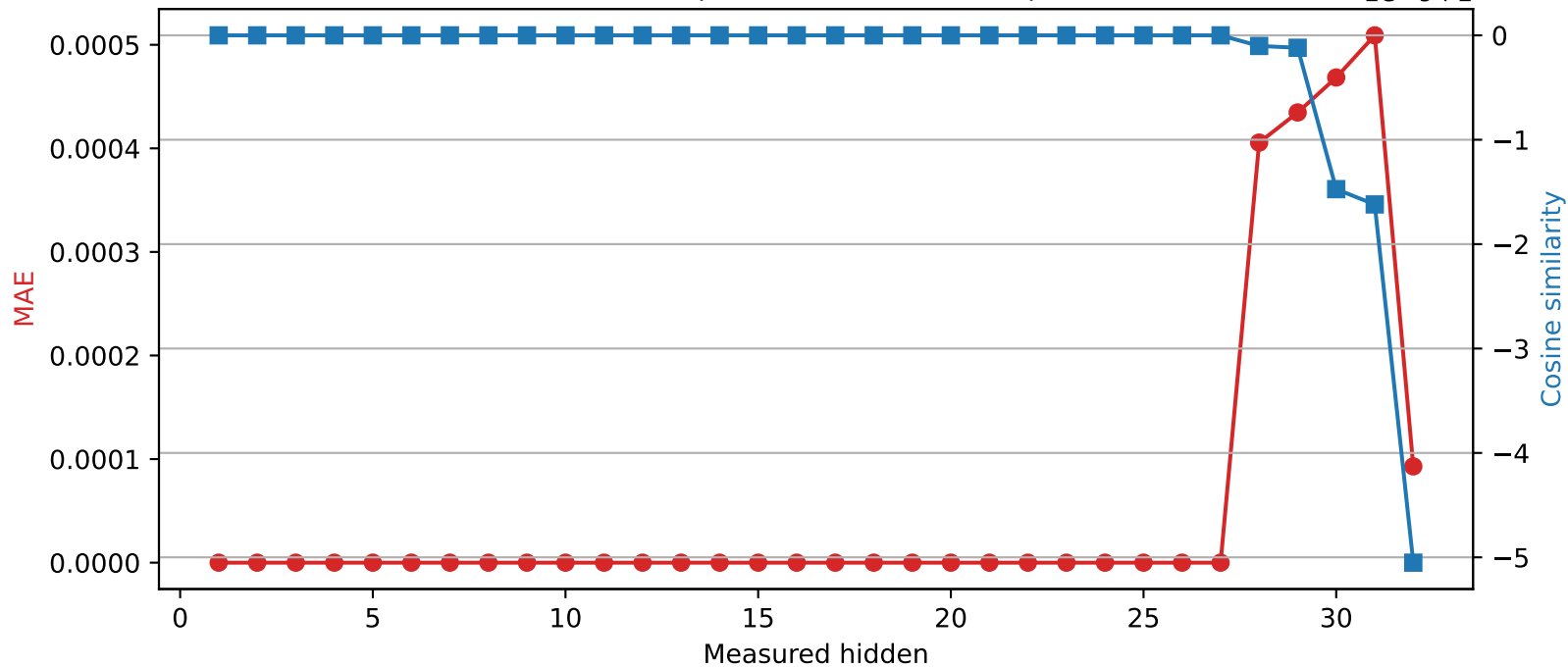
Phi-3-mini-4k-instruct | Quantized layer 27 | float32 \rightarrow int16
