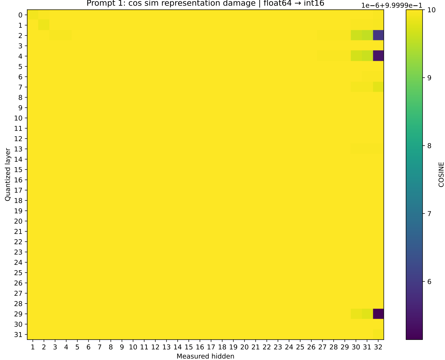
Phi-3-mini-4k-instruct Prompt 1: cos sim representation damage | float64 → int16
