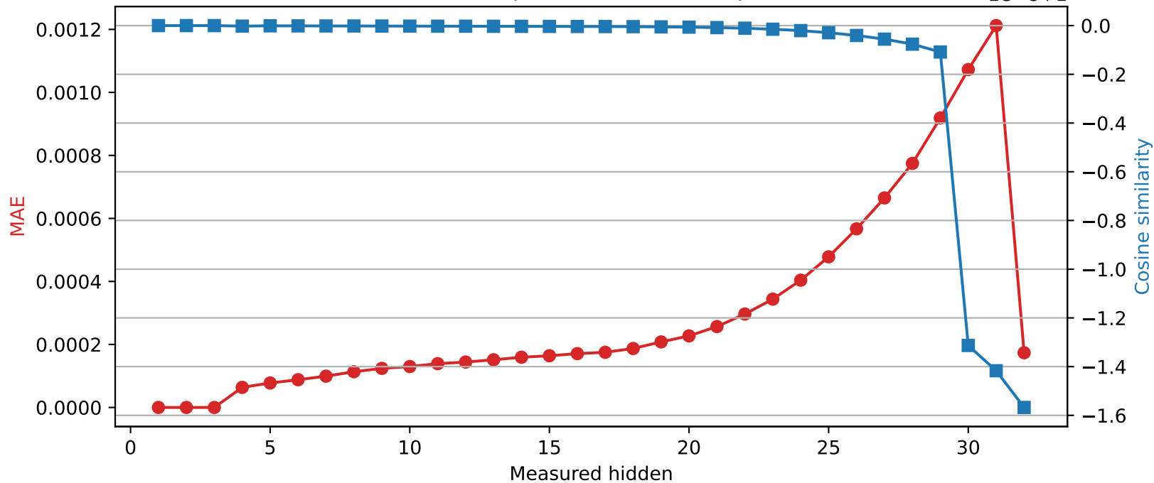
Phi-3-mini-4k-instruct | Quantized layer 3 | float64 \rightarrow int16
