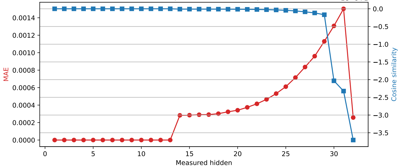
Phi-3-mini-4k-instruct | Quantized layer 13 | float64 → int16
