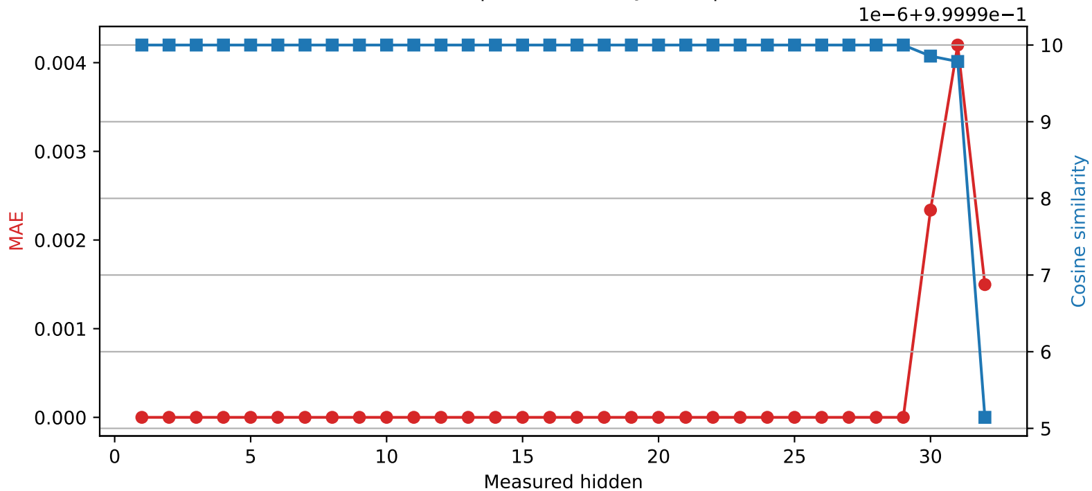
Phi-3-mini-4k-instruct | Quantized layer 29 | float64 → int16
