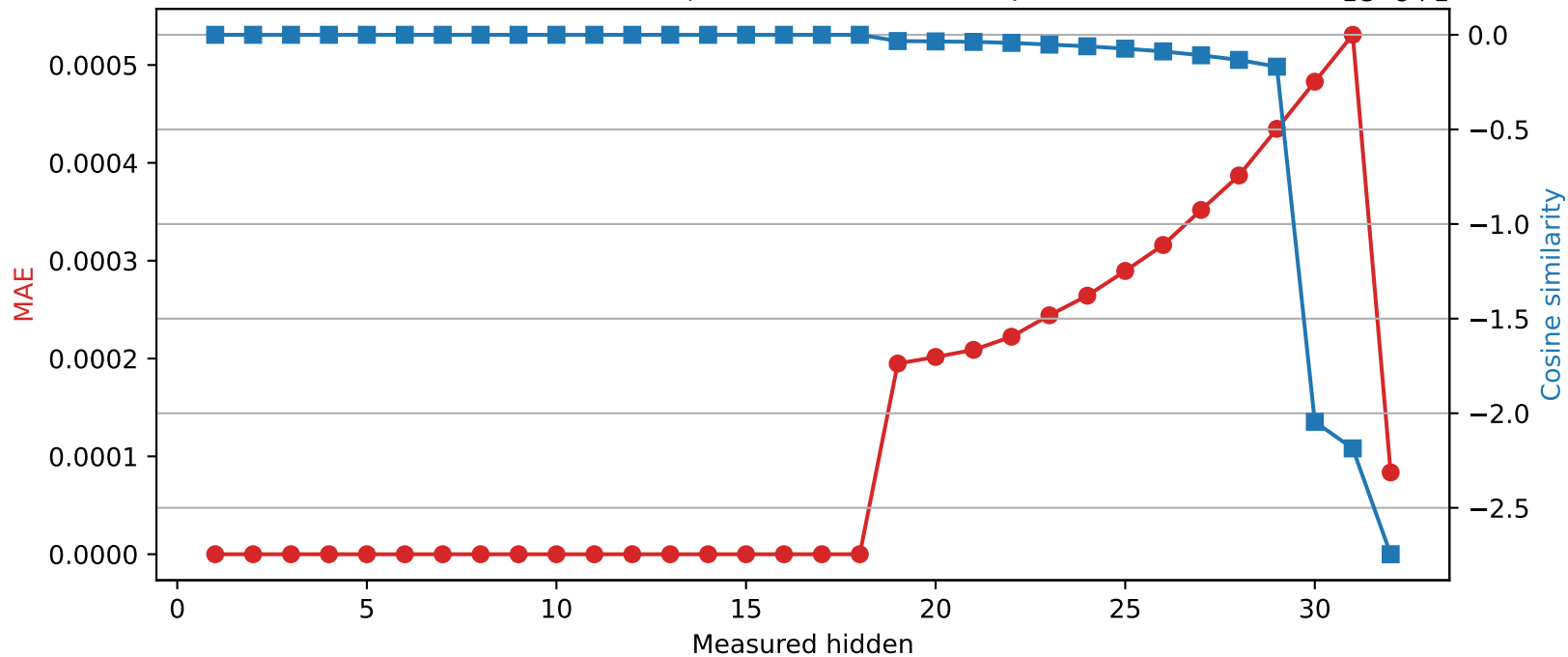
Phi-3-mini-4k-instruct | Quantized layer 18 | float64 \rightarrow int16
