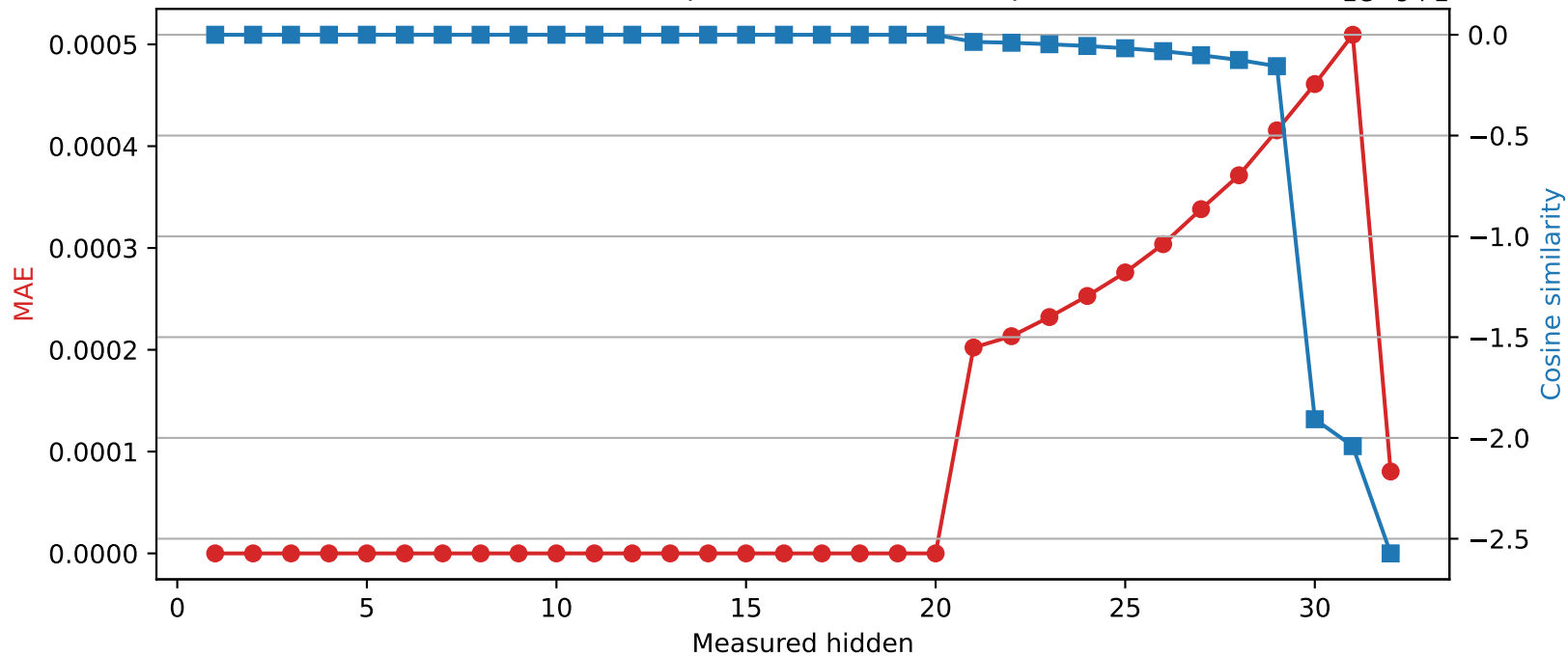
Phi-3-mini-4k-instruct | Quantized layer 20 | float64 \rightarrow int16
