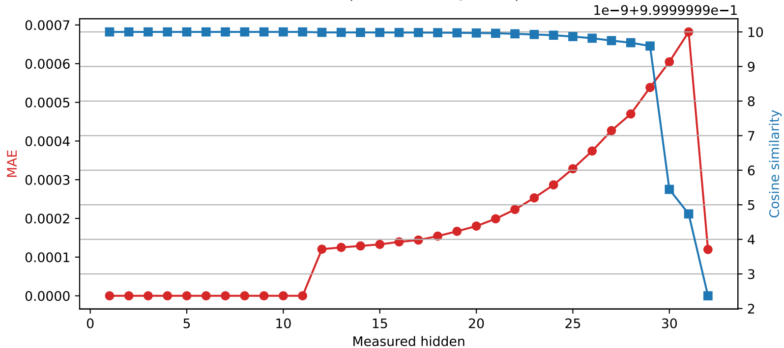
Phi-3-mini-4k-instruct | Quantized layer 11 | float64 → int16
