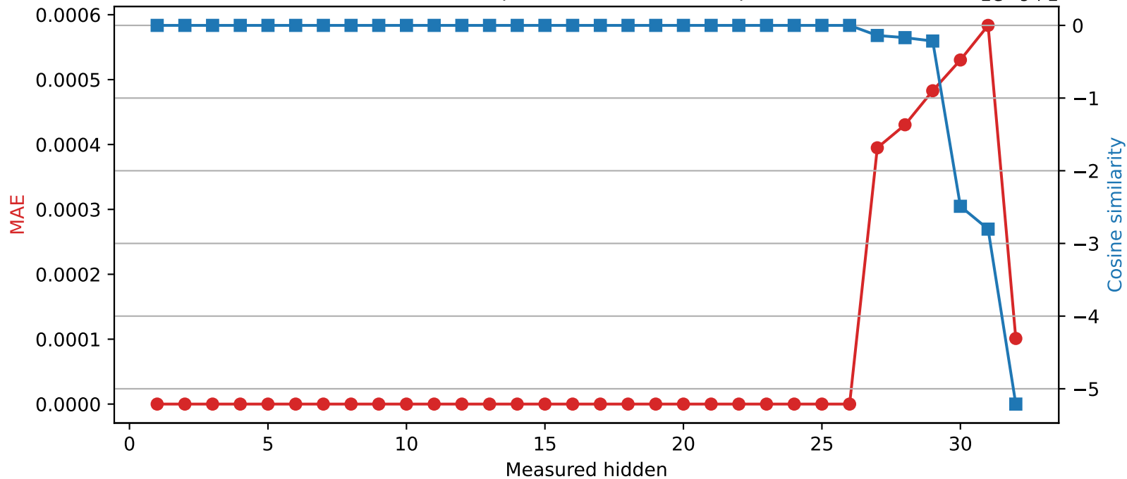
Phi-3-mini-4k-instruct | Quantized layer 26 | float64 \rightarrow int16
