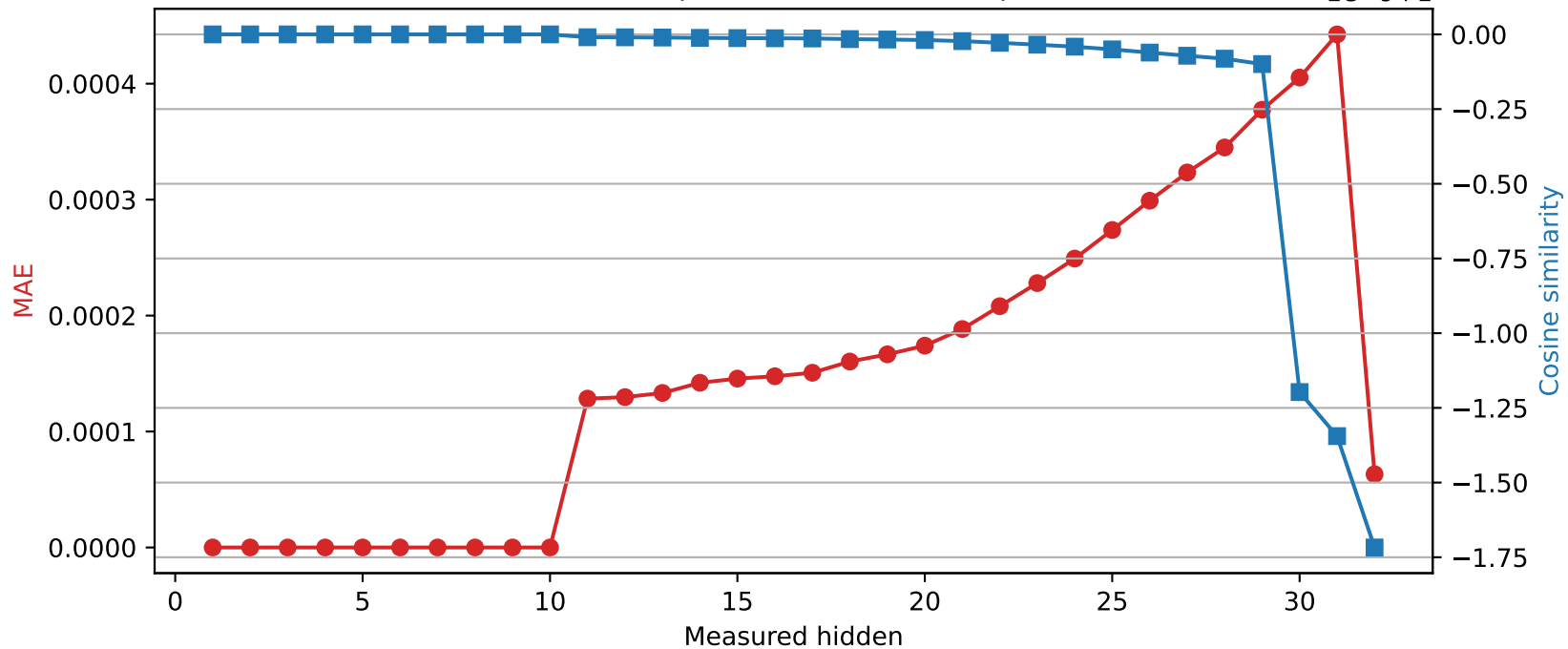
Phi-3-mini-4k-instruct | Quantized layer 10 | float64 → int16
