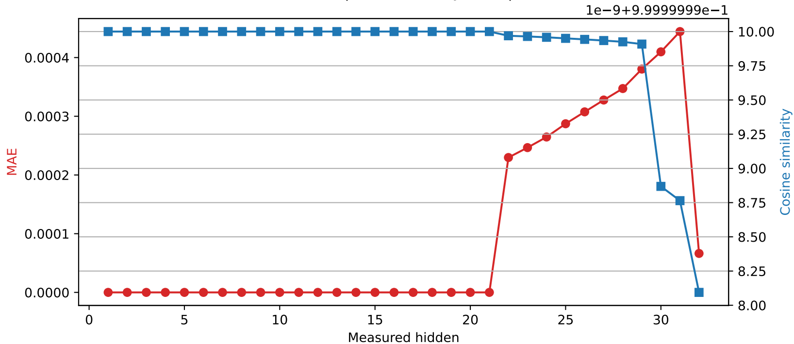
Phi-3-mini-4k-instruct | Quantized layer 21 | float64 → int16
