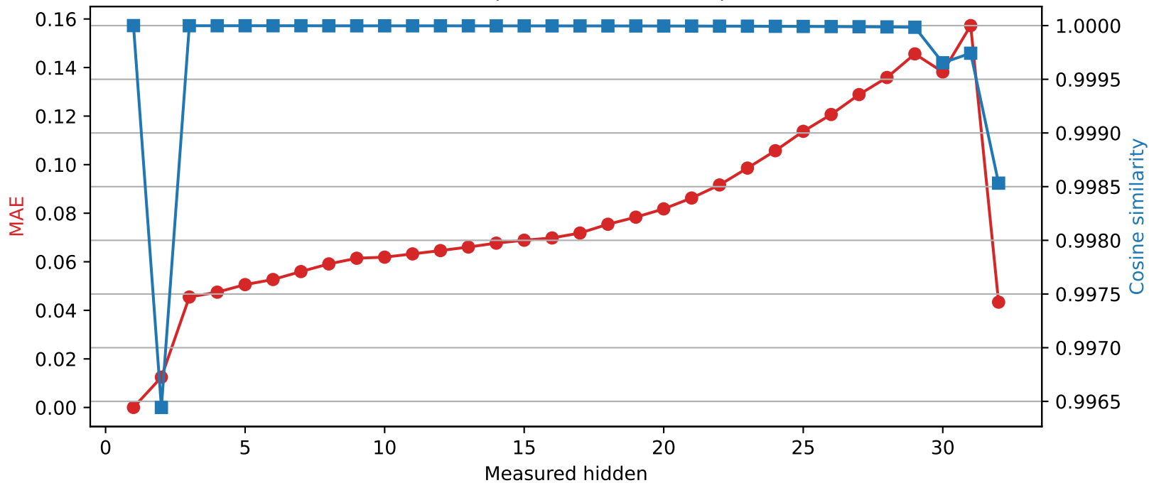
Phi-3-mini-4k-instruct | Quantized layer 1 | float16 \rightarrow int8
